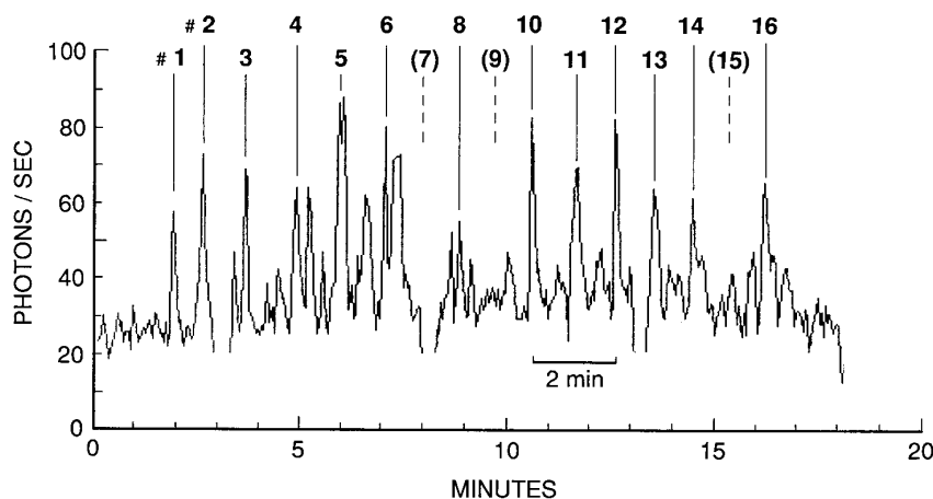
Fig. 8. Calcium spiking shows some clear periodicity. This figure expands part of Fig. 6l, which shows the time course of luminescence from the anterior high calcium zone of a static slug. The eight spikes labelled with even numbers have an average period of 2.0 minutes; while the six marked 1, 3, 5, 11, 13 and (15) can be thought of as an incomplete run of eight others, which have an average period of 1.9 minutes. Together, these 13-14 spikes can be thought of as defining a second harmonic with a period of 1.0 minutes.
